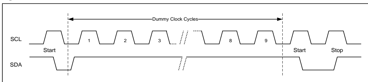
Figure 4-4 Soft Reset
