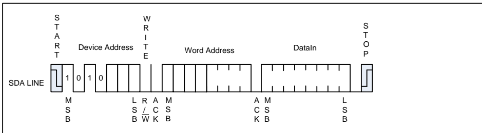
Figure 5-1 Byte Write
