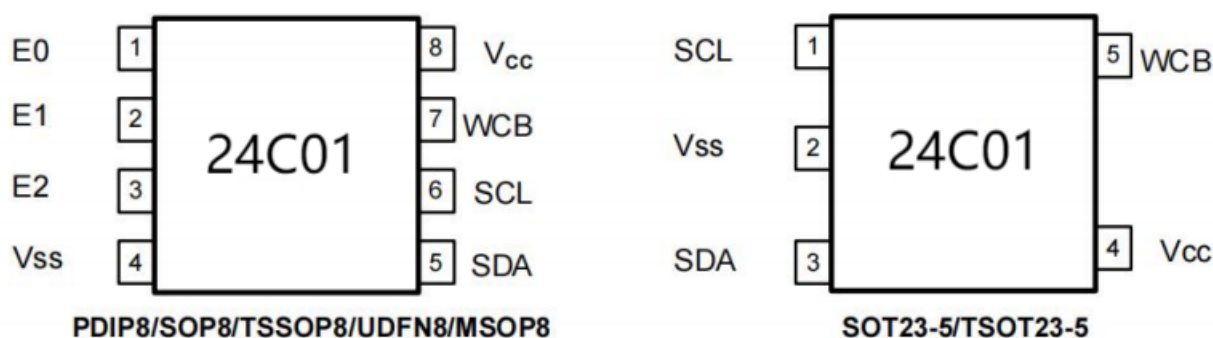
Figure 2-1 Pin Configuration
