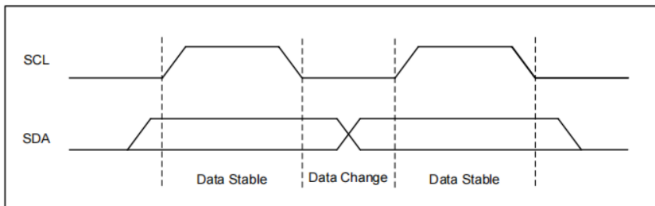
Figure 5-1 Data Validity
