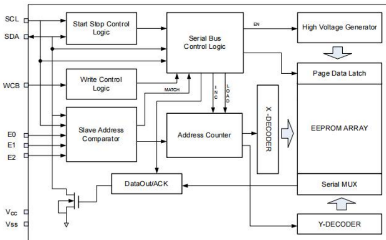
Figure 3-1 Block Diagram
