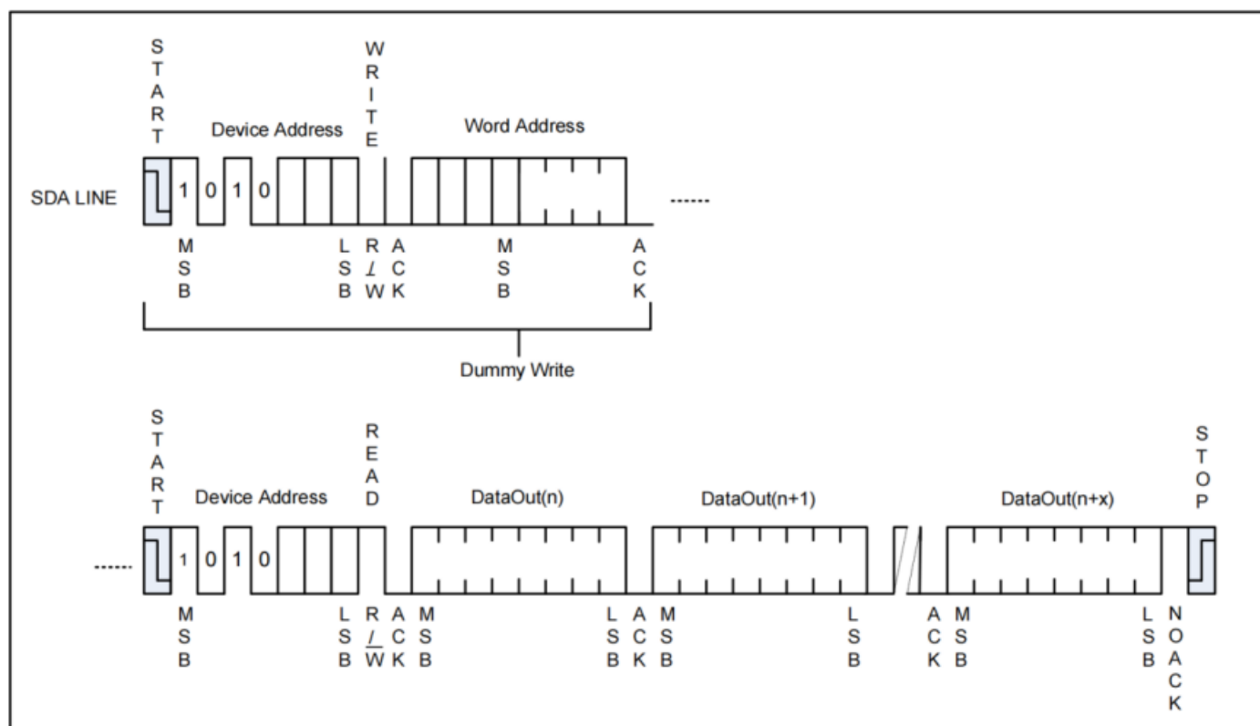
Figure 6-5 Sequential Read
