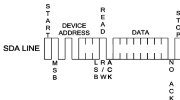
Figure 5: Current Address Read
