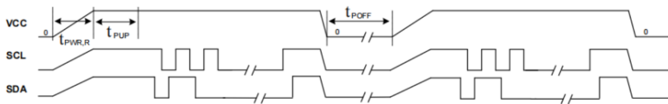
Figure 11: Power on and Power down
