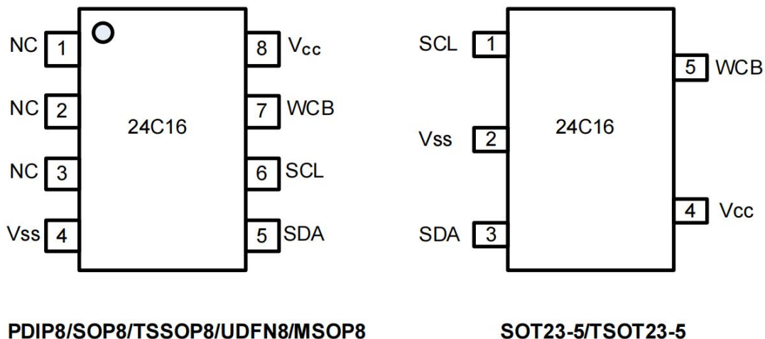
Figure 1-1 Pin Configuration
