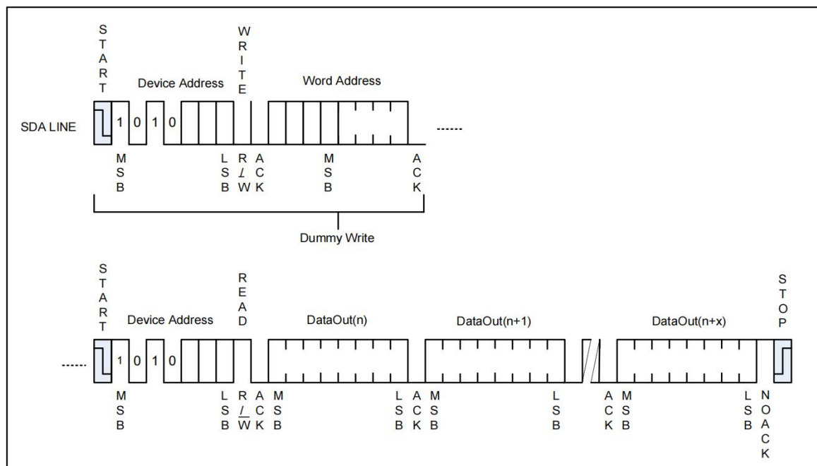
Figure 5-5 Sequential Read
