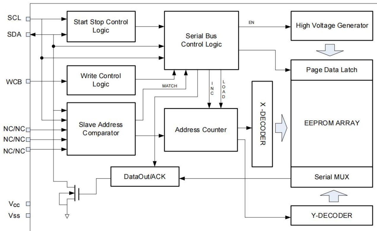
Figure 2-1 Block Diagram
