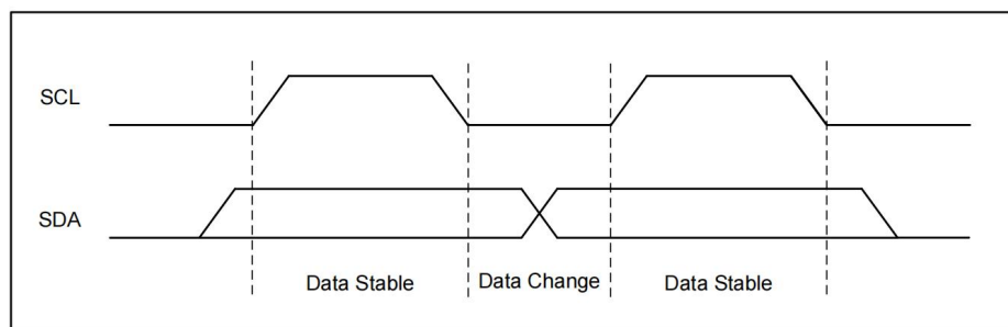
Figure 4-1 Data Validity
