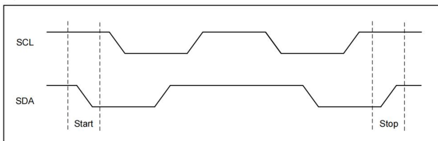
Figure 4-2 Start and Stop Definition
