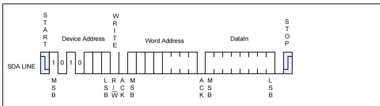
Figure 5-1 Byte Write
