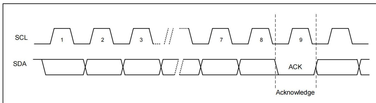
Figure 4-3 Output Acknowledge
