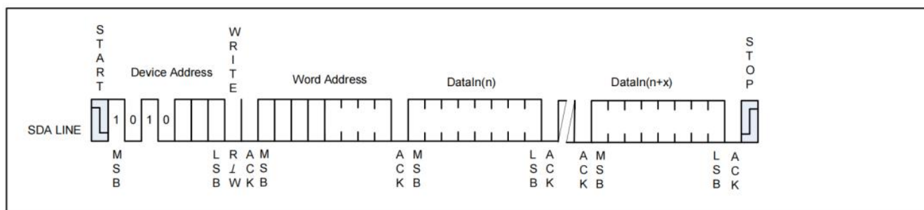
Figure 5-2 Page Write
