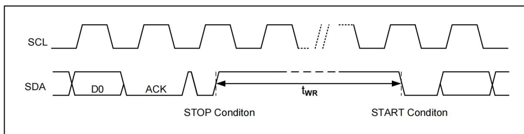
Figure 3-2 Write Cycle Timing
