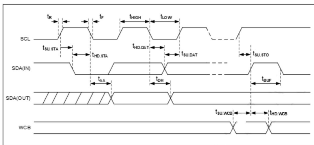
Figure 3-2 Write Cycle Timing
