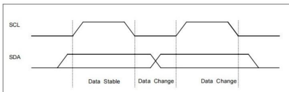
Figure 5-1 Data Validity
