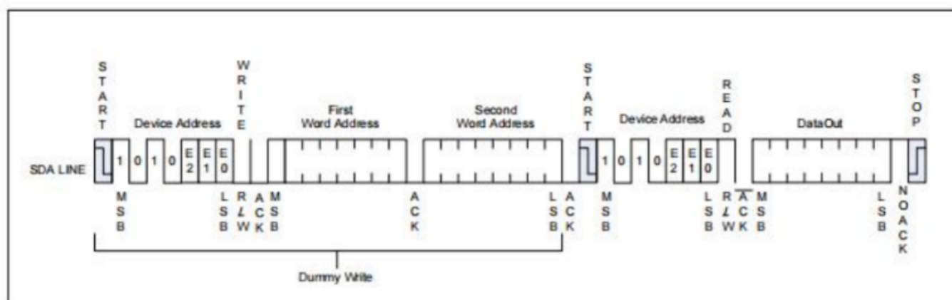
Figure 6-4 Random Read
