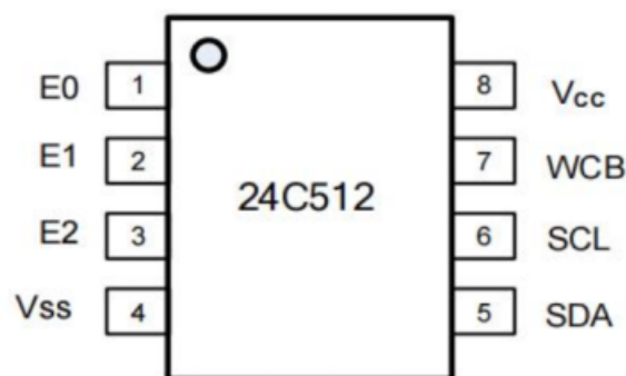
Figure 1-1 Pin Configuration
