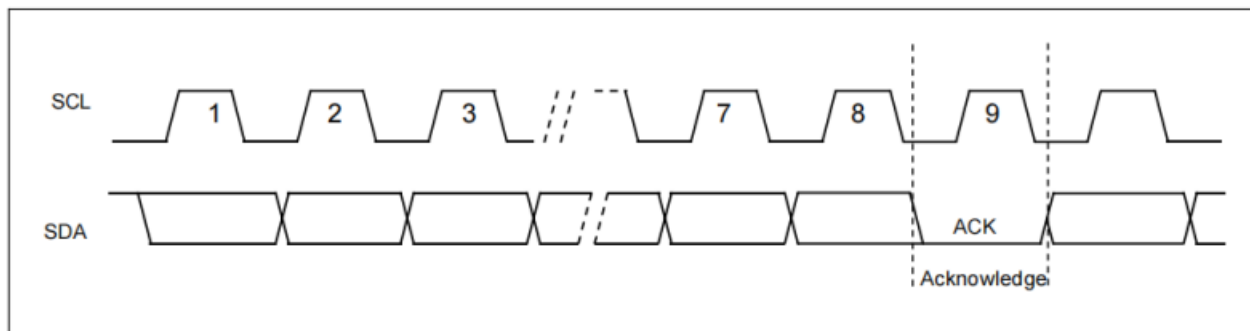
Figure 4-3 Output Acknowledge
