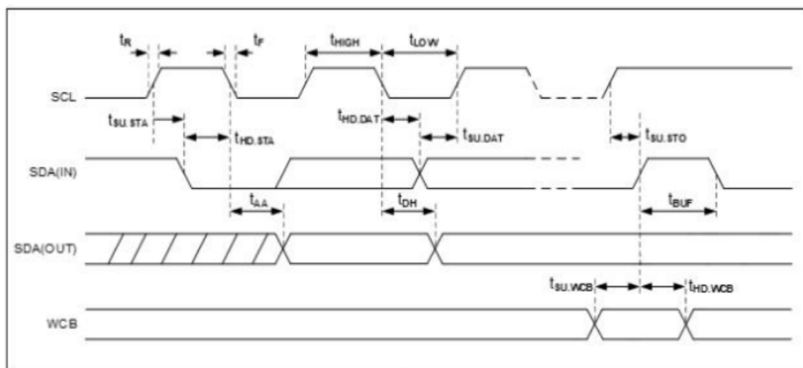
Figure Write Cycle Timing
