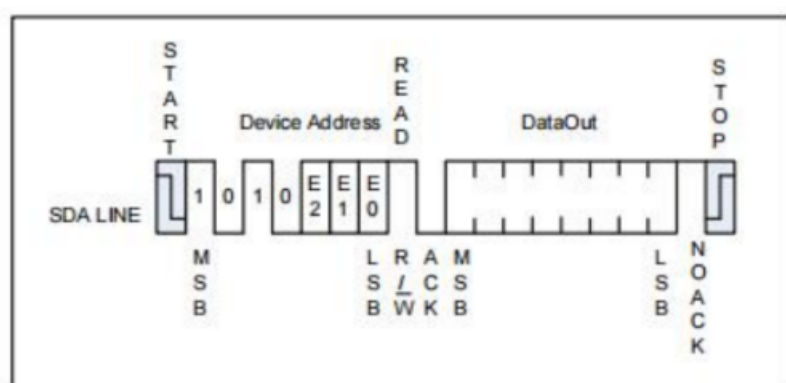
Figure 6-3 Current Address Read
