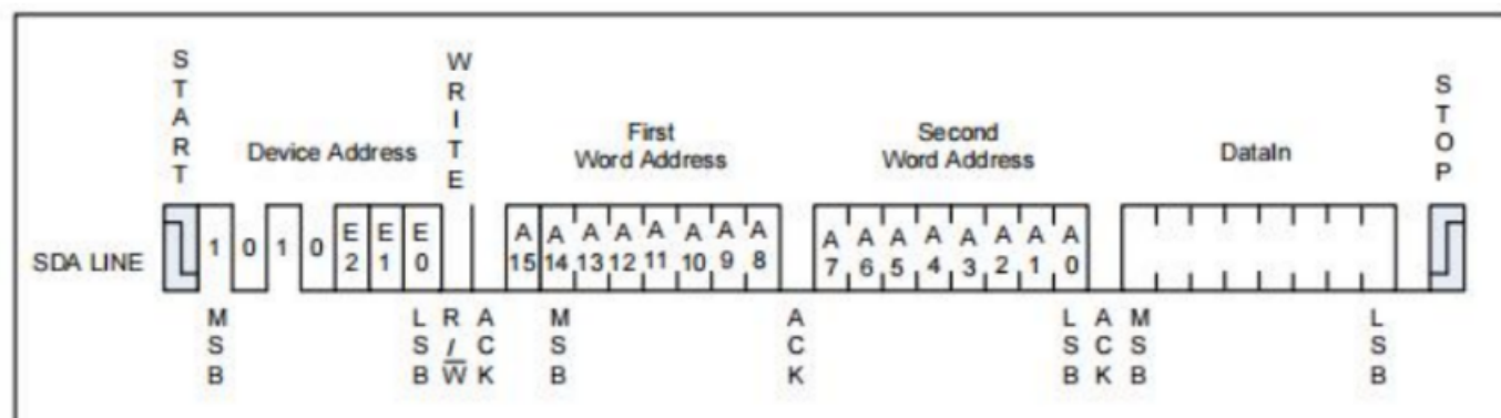
Figure 6-1 Byte Write
