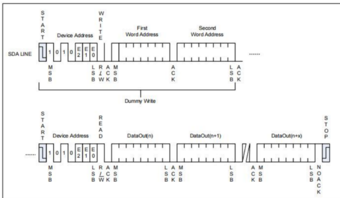
Figure 6-5 Sequential Read
