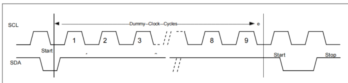
Figure 5-4 Soft Reset
