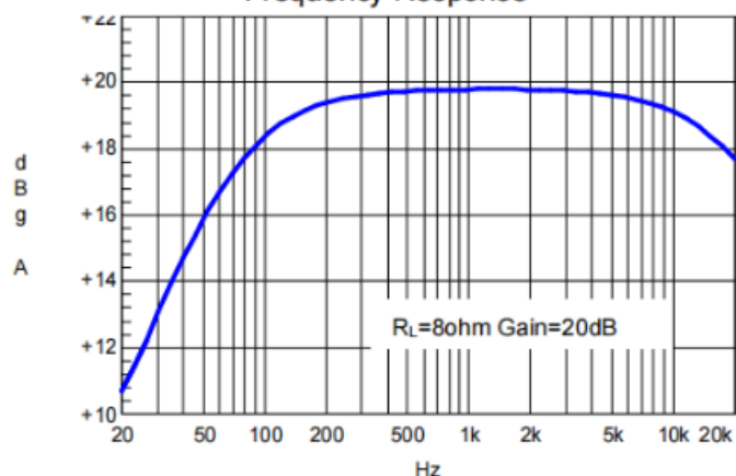
Frequency Response
