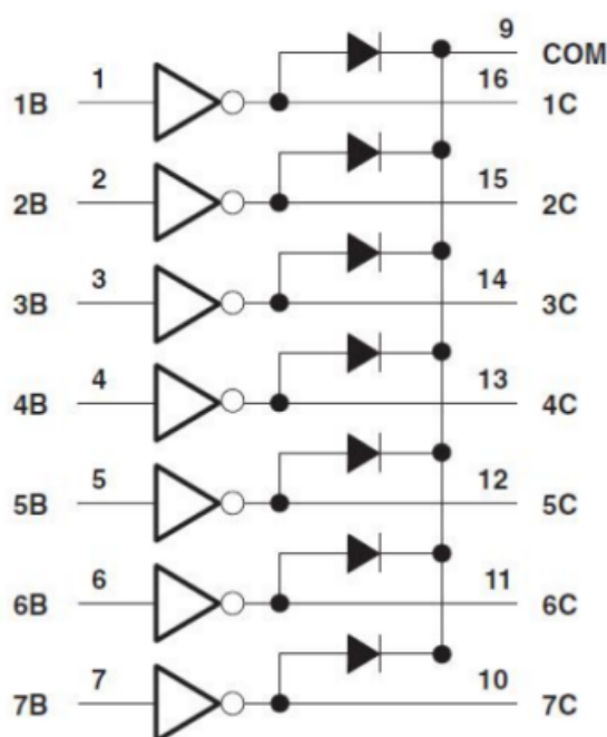
LOGIC DIAGRAM
