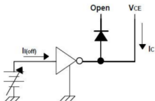
Fig.3 Ii(off) Test Circuit
